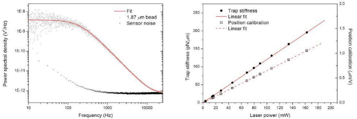
Figure 12. Power spectral density of the Brownian motion of a trapped microsphere (1.87 \mu\text{m} ) and of the sensor noise (left). Trap stiffness and position calibration are linear with laser power once the effect of the laser heating is corrected (right).
