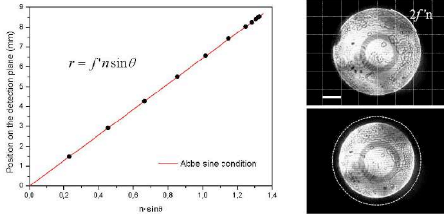
Figure 5. The calibration of the BFP of the collecting lens shows that the instrument perfectly follows the Abbe sine condition. The calibration provides a measurement of the solid angle captured by the system, which can be used to correctly set the position of the sensor. (Top) NA \sim n . (Bottom) NA < n . The scale bar corresponds to an effective NA of 0.5.
